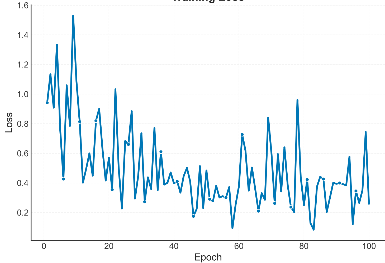
Training Loss
