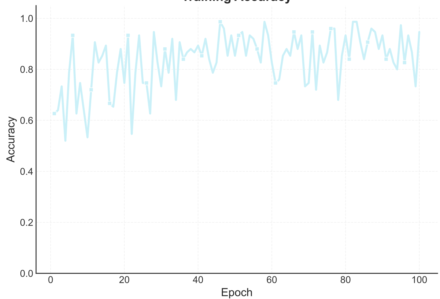
Training Accuracy
